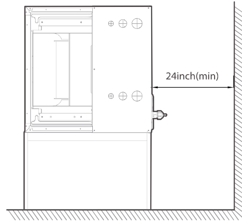
Horizontal installations
